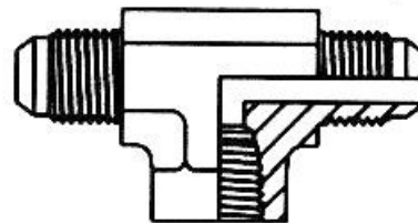
FEMALE BRANCH TEE
