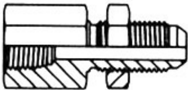
FEMALE BULKHEAD CONNECTOR
